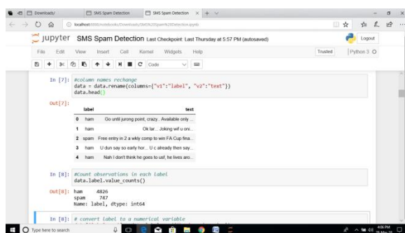
Fig.4.2.SMS Spam detection.
